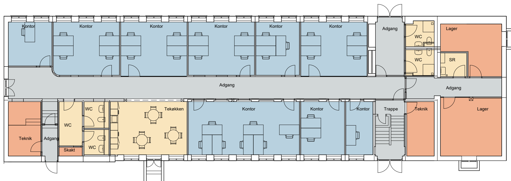
Ground floor
